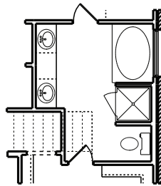
OPT. MASTER BATH OPT. MASTER BATH AND SHOWER
